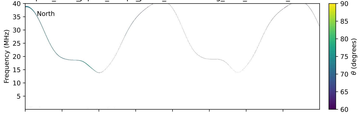
expres_earth_jupiter_europa_jrm33_lossc-wid1deg_3kev_20120405_v11.cdf
