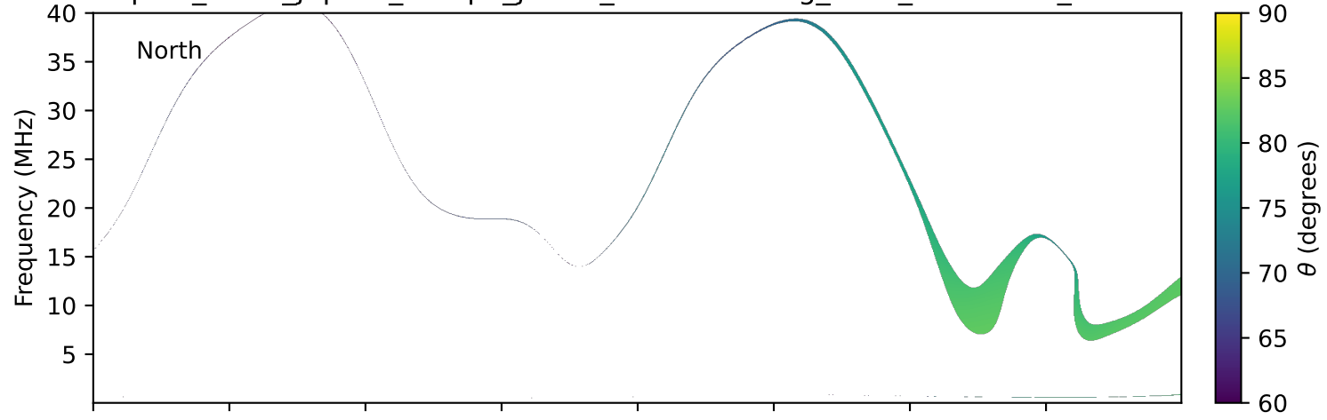
expres_earth_jupiter_europa_jrm33_lossc-wid1deg_3kev_20120402_v11.cdf
