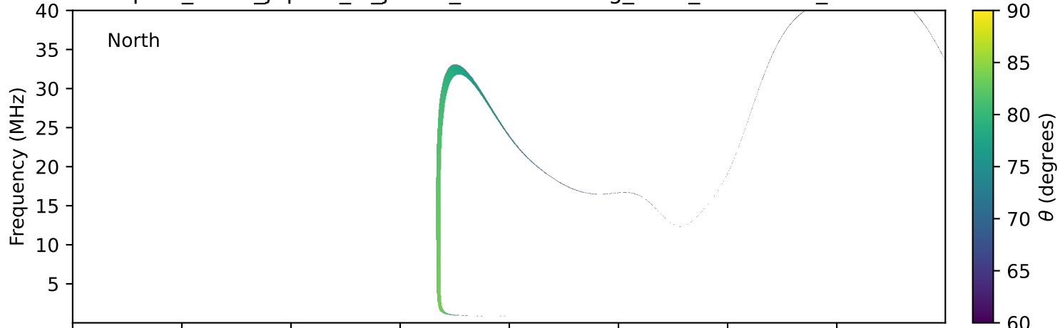
expres_earth_jupiter_io_jrm33_lossc-wid1deg_3kev_20120324_v11.cdf
