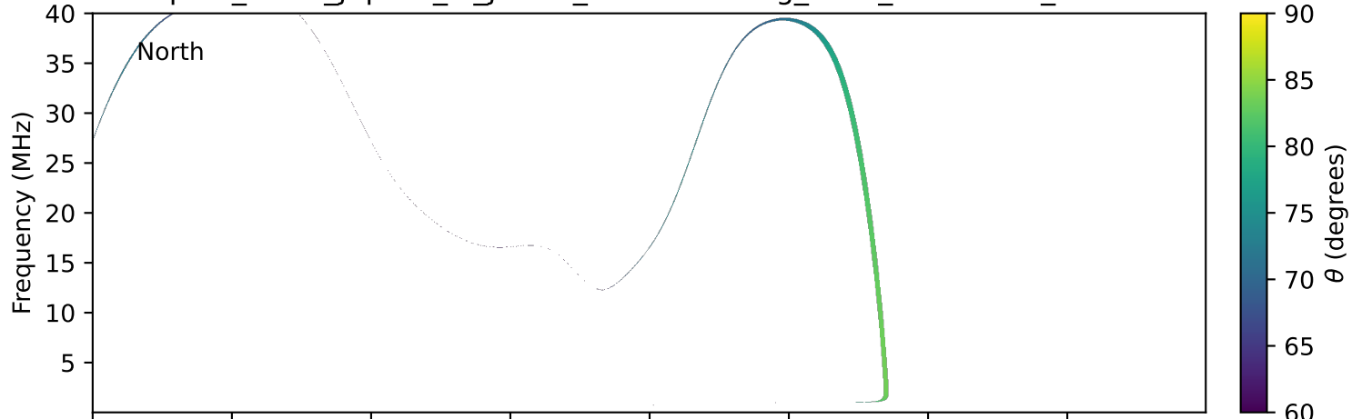
expres_earth_jupiter_io_jrm33_lossc-wid1deg_3kev_20120321_v11.cdf
