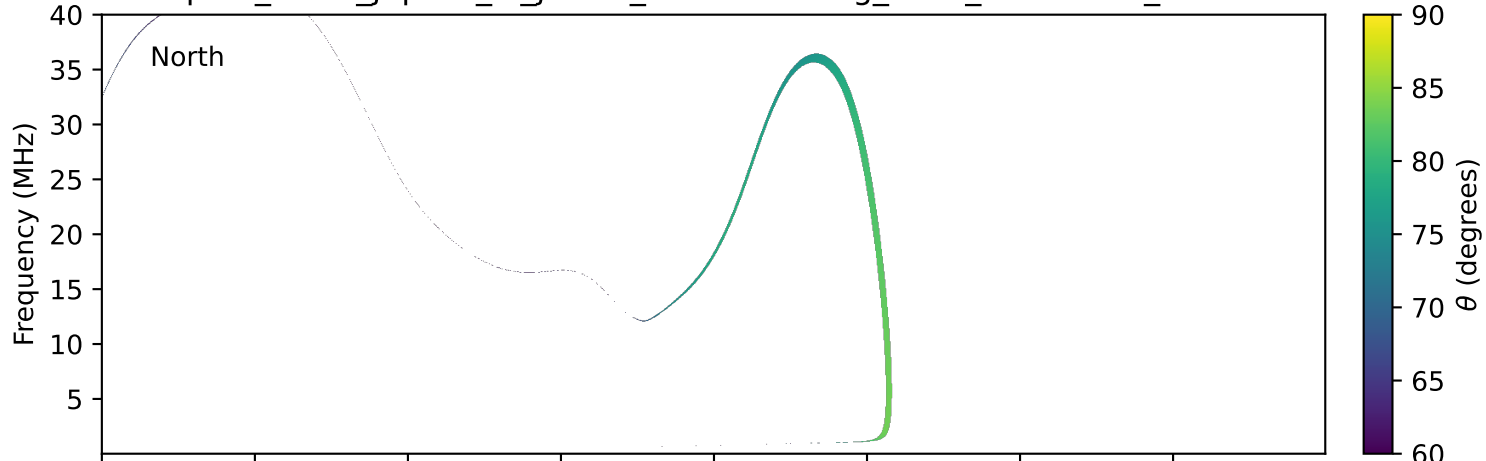
expres_earth_jupiter_io_jrm33_lossc-wid1deg_3kev_20120314_v11.cdf
