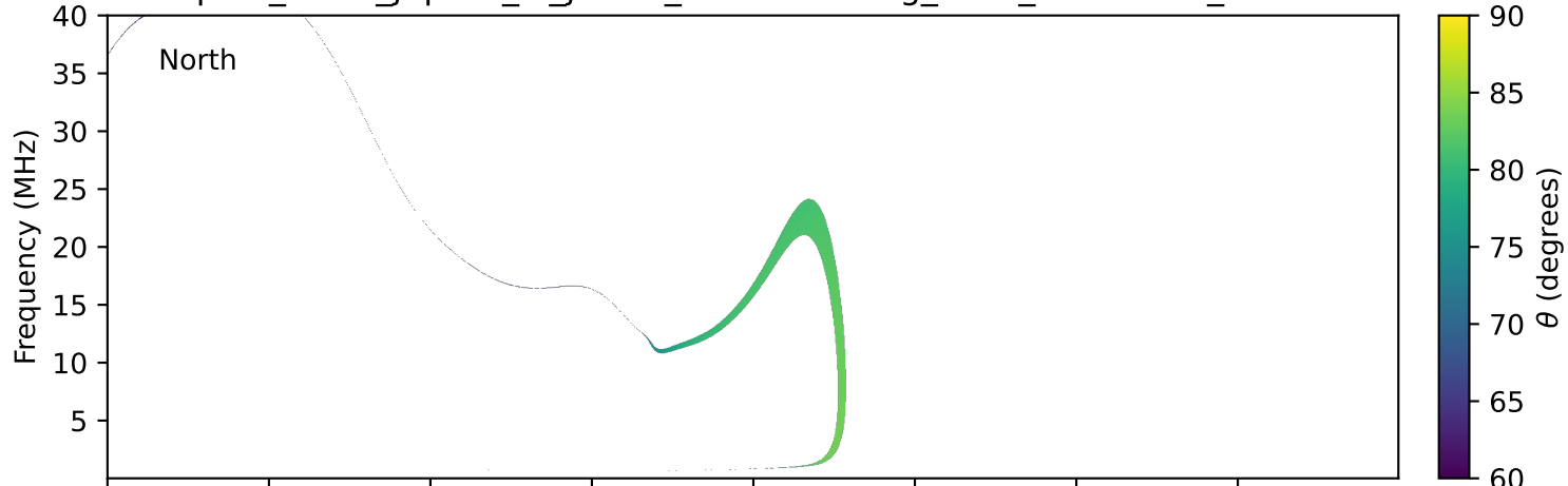
expres_earth_jupiter_io_jrm33_lossc-wid1deg_3kev_20120307_v11.cdf
