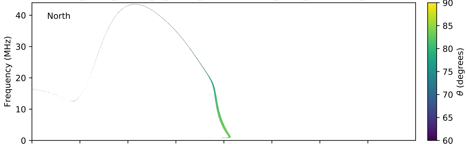
expres_earth_jupiter_io_jrm09_lossc-wid1deg_3kev_20120330_v01.cdf
