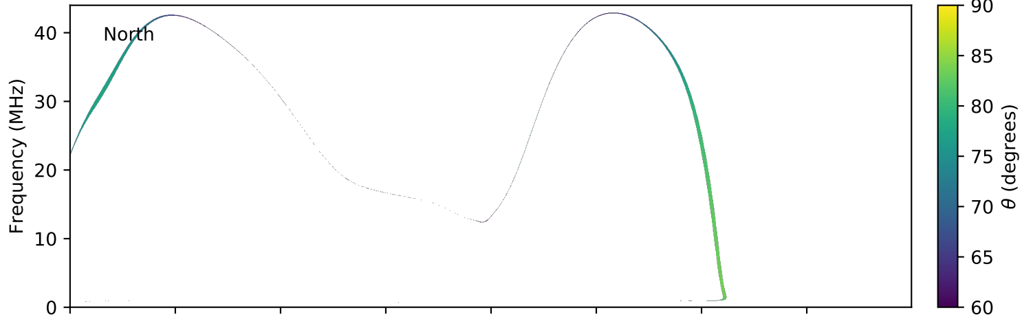
expres_earth_jupiter_io_jrm09_lossc-wid1deg_3kev_20120328_v01.cdf
