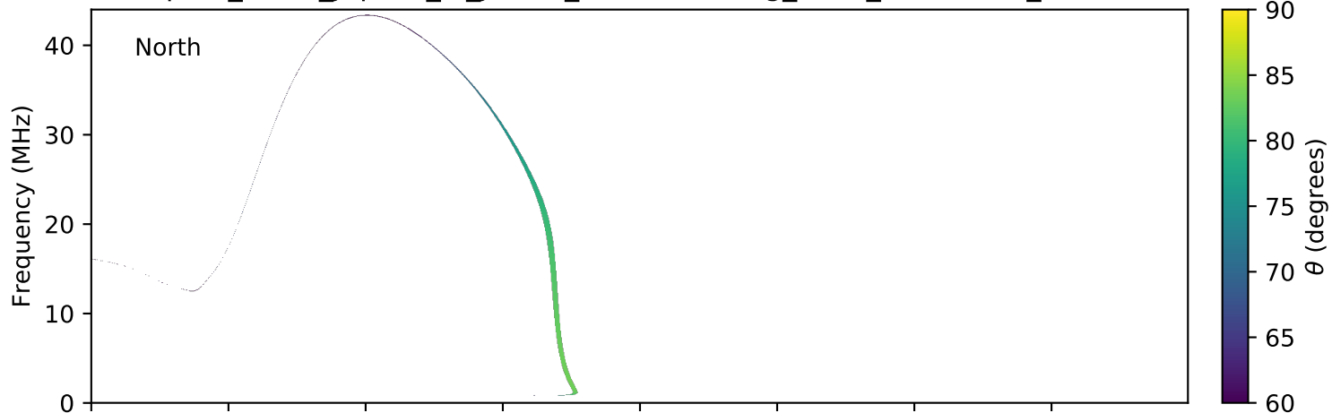
expres_earth_jupiter_io_jrm09_lossc-wid1deg_3kev_20120323_v01.cdf
