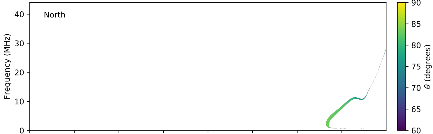
expres_earth_jupiter_io_jrm09_lossc-wid1deg_3kev_20120320_v01.cdf
