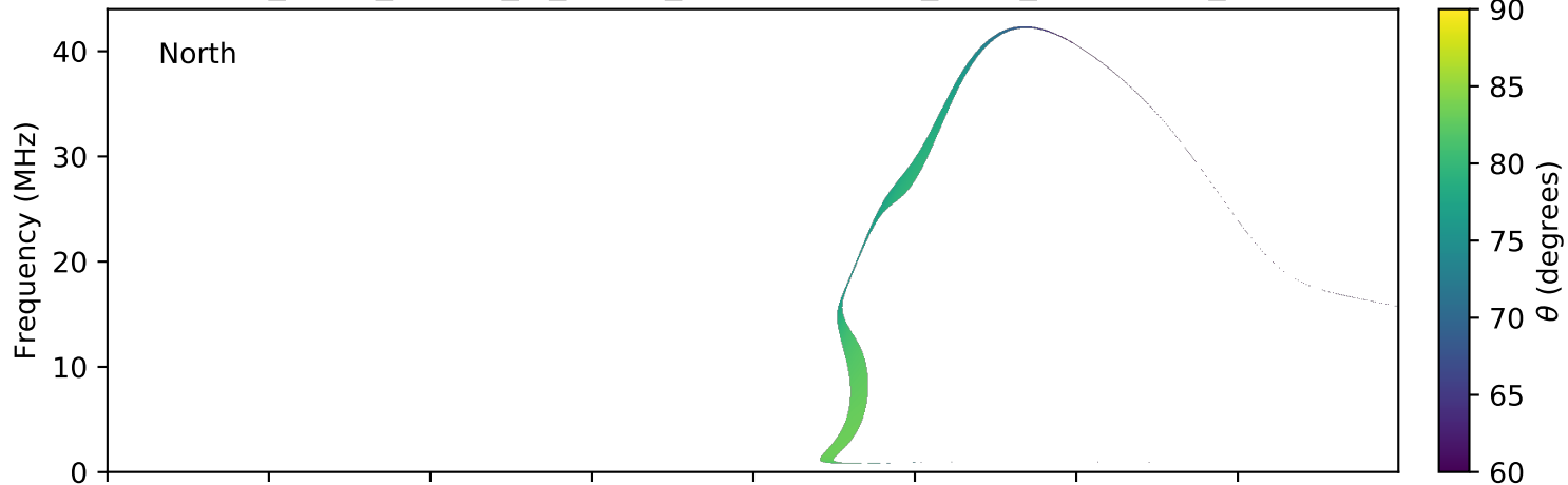
expres_earth_jupiter_io_jrm09_lossc-wid1deg_3kev_20120315_v01.cdf
