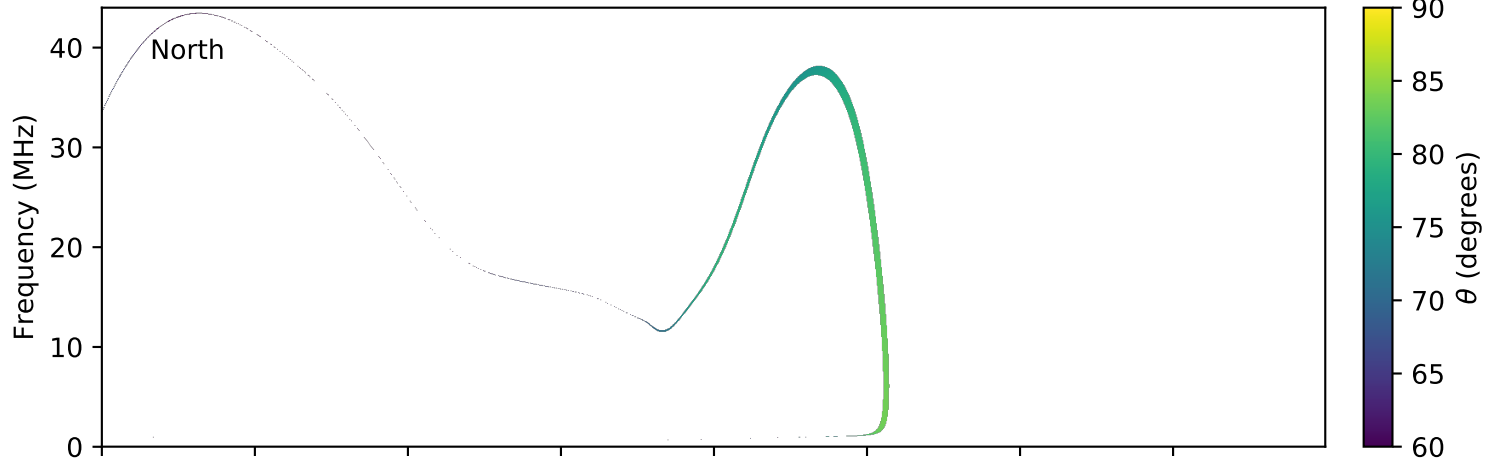
expres_earth_jupiter_io_jrm09_lossc-wid1deg_3kev_20120314_v01.cdf
