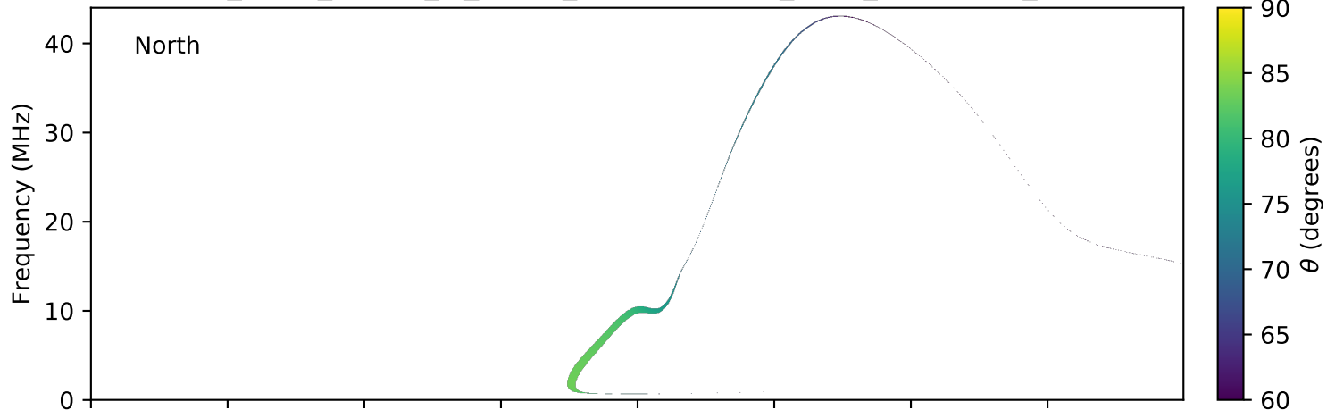
expres_earth_jupiter_io_jrm09_lossc-wid1deg_3kev_20120308_v01.cdf
