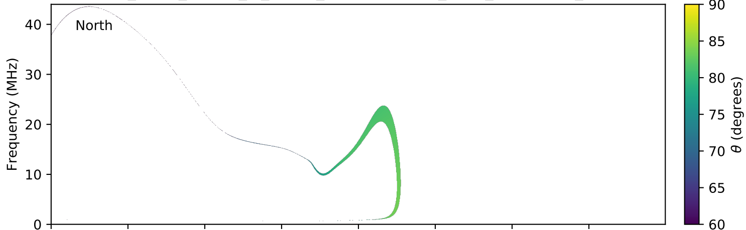
expres_earth_jupiter_io_jrm09_lossc-wid1deg_3kev_20120307_v01.cdf
