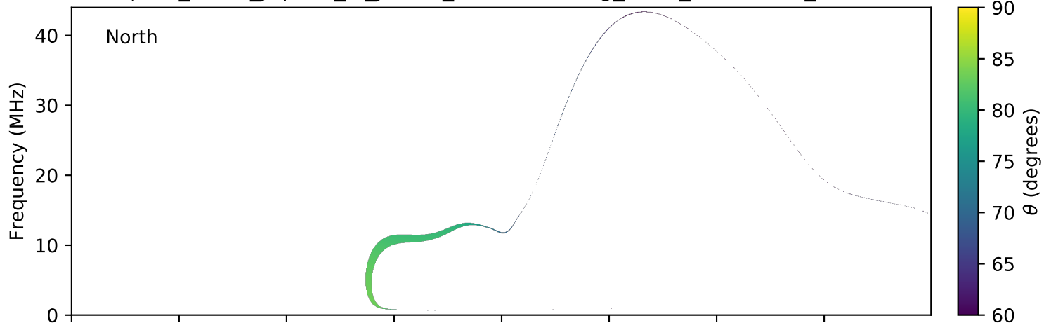
expres_earth_jupiter_io_jrm09_lossc-wid1deg_3kev_20120301_v01.cdf
