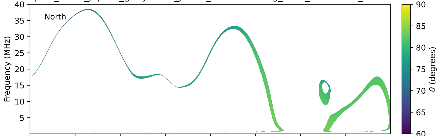
expres_earth_jupiter_ganymede_jrm33_lossc-wid1deg_3kev_20120331_v11.cdf
