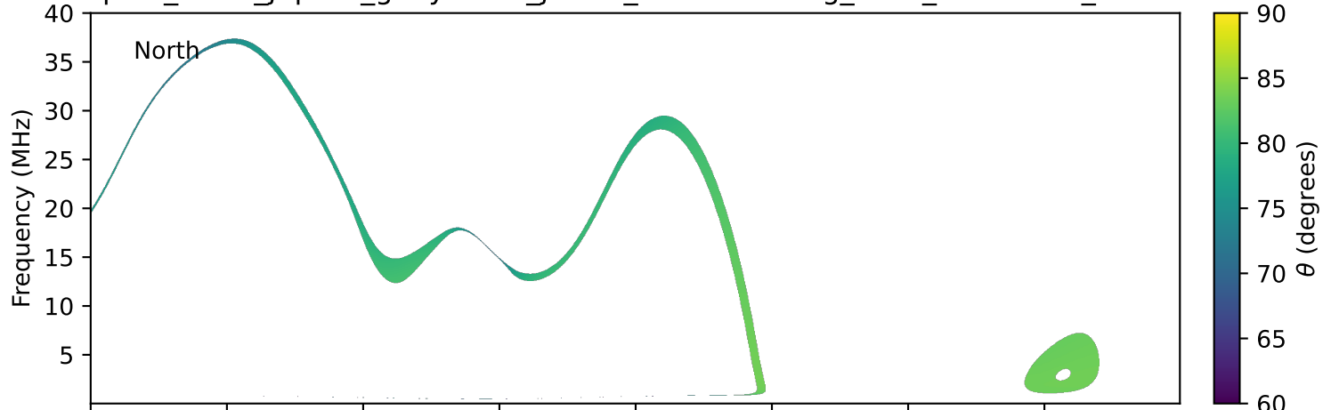
expres_earth_jupiter_ganymede_jrm33_lossc-wid1deg_3kev_20120324_v11.cdf
