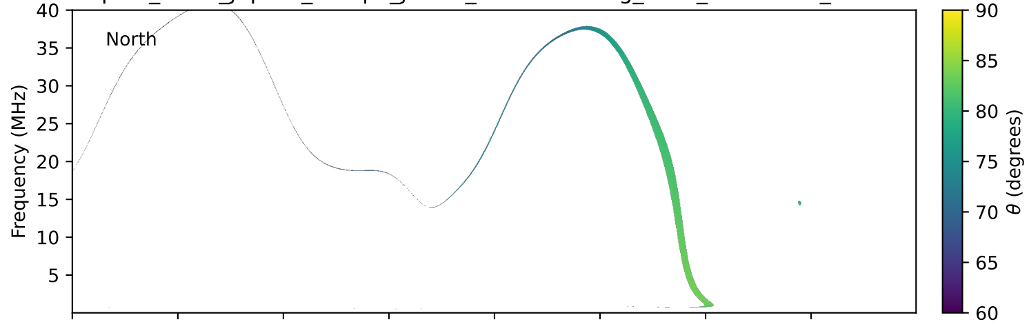
expres_earth_jupiter_europa_jrm33_lossc-wid1deg_3kev_20120326_v11.cdf
