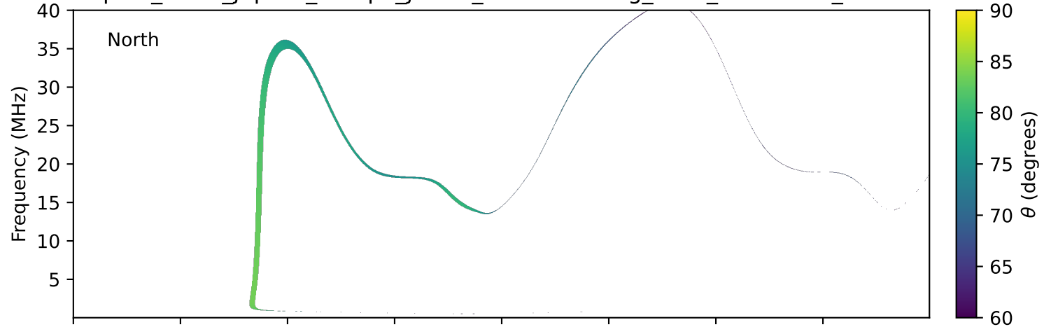
expres_earth_jupiter_europa_jrm33_lossc-wid1deg_3kev_20120325_v11.cdf
