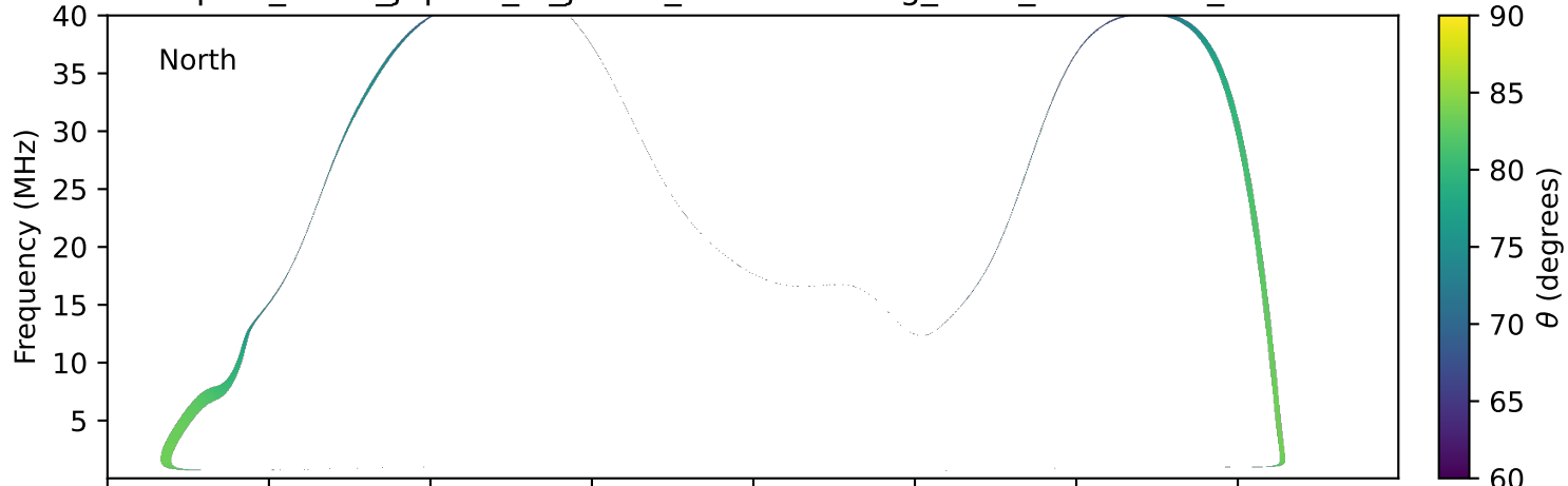
expres_earth_jupiter_io_jrm33_lossc-wid1deg_3kev_20120225_v11.cdf
