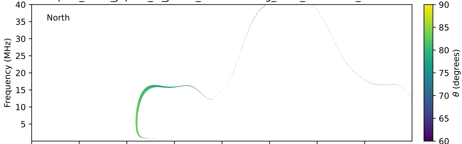
expres_earth_jupiter_io_jrm33_lossc-wid1deg_3kev_20120223_v11.cdf
