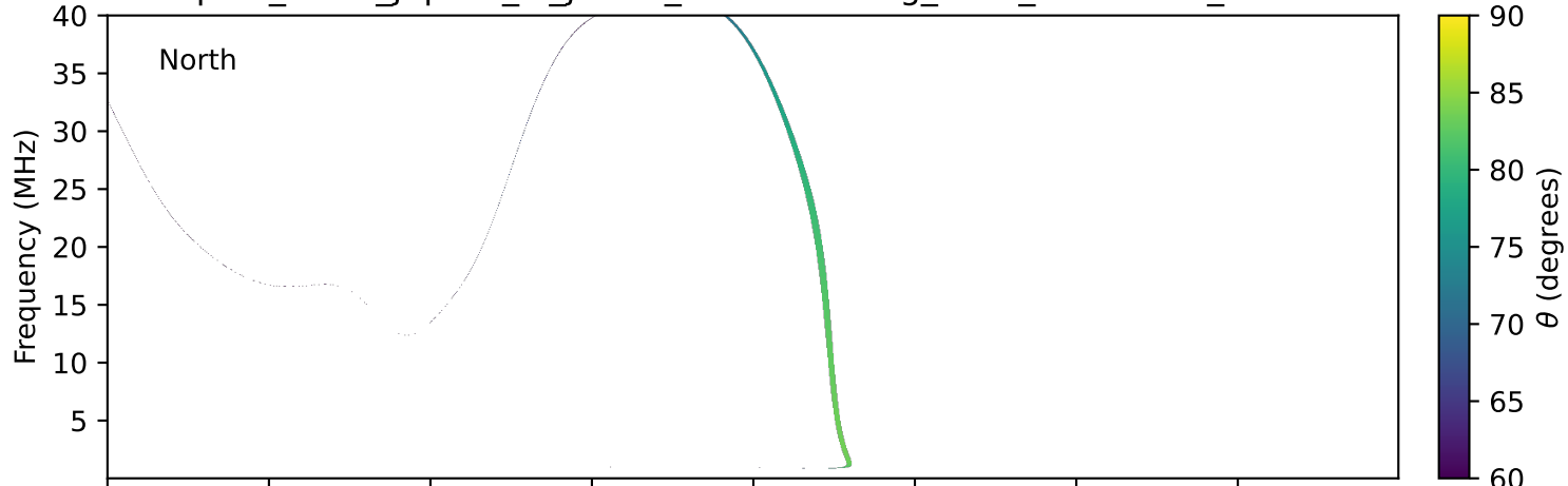
expres_earth_jupiter_io_jrm33_lossc-wid1deg_3kev_20120220_v11.cdf
