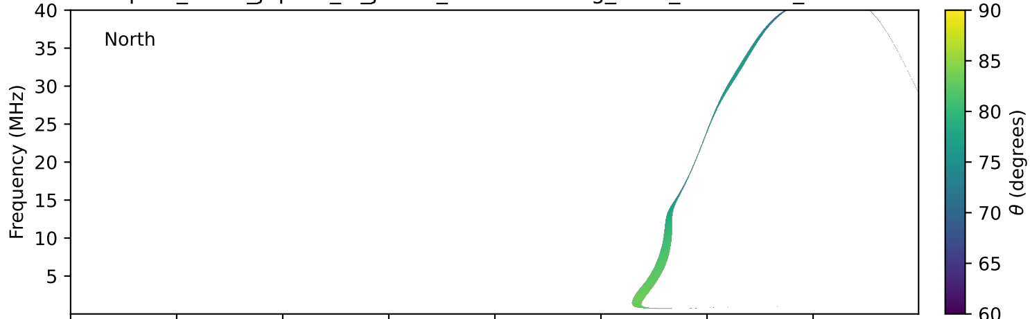
expres_earth_jupiter_io_jrm33_lossc-wid1deg_3kev_20120212_v11.cdf
