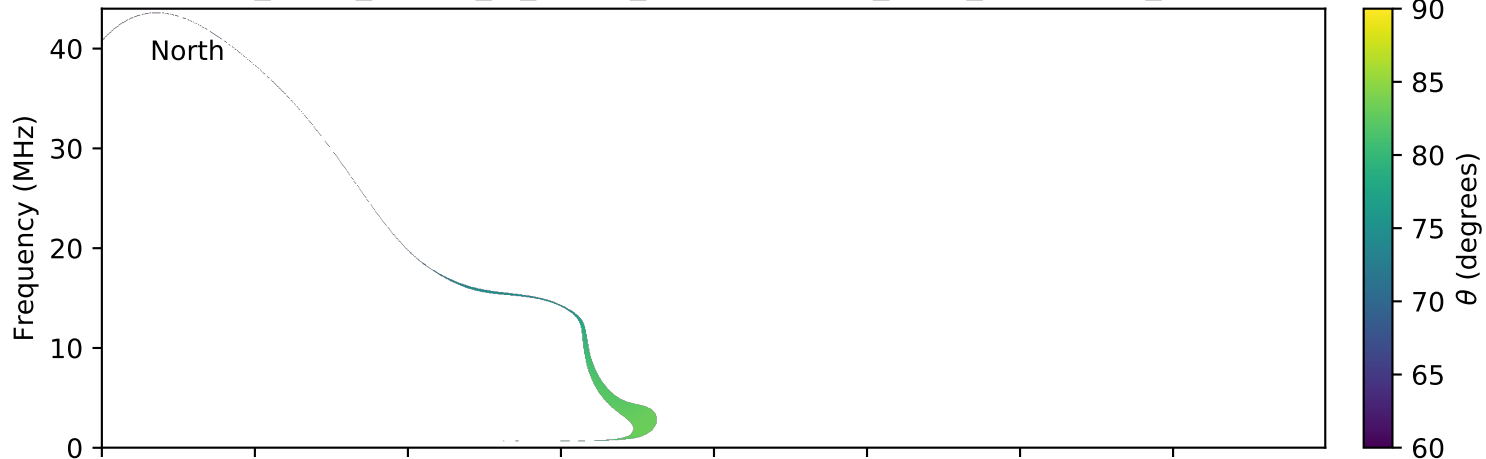
expres_earth_jupiter_io_jrm09_lossc-wid1deg_3kev_20120229_v01.cdf
