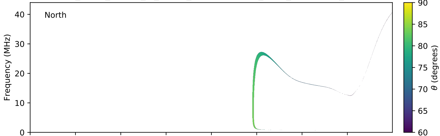
expres_earth_jupiter_io_jrm09_lossc-wid1deg_3kev_20120228_v01.cdf
