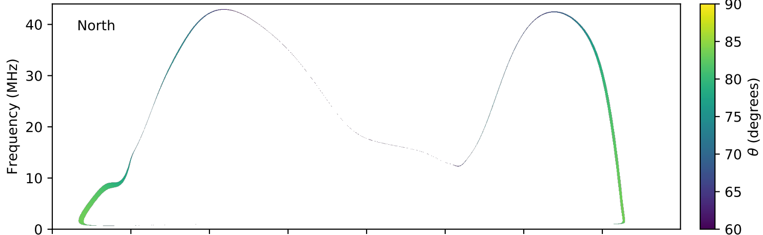
expres_earth_jupiter_io_jrm09_lossc-wid1deg_3kev_20120225_v01.cdf
