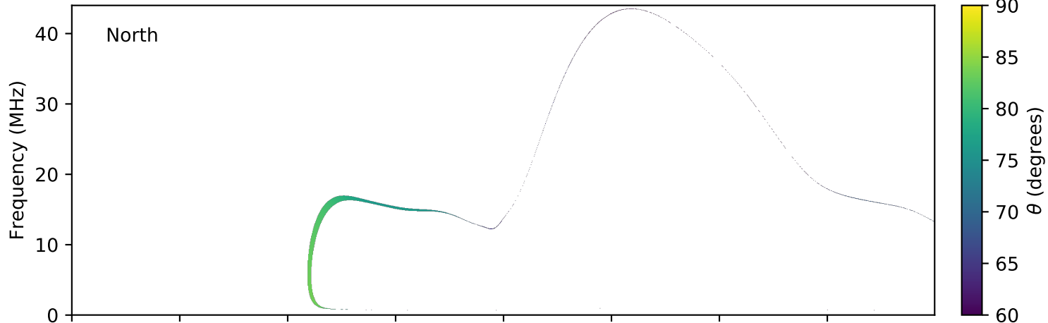
expres_earth_jupiter_io_jrm09_lossc-wid1deg_3kev_20120223_v01.cdf
