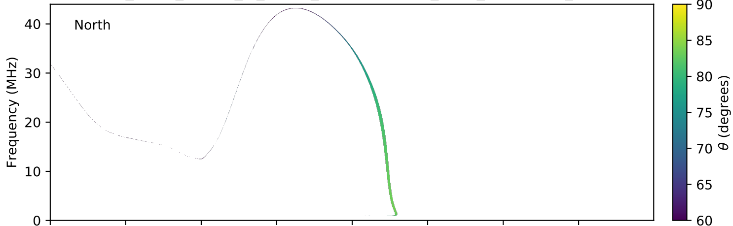
expres_earth_jupiter_io_jrm09_lossc-wid1deg_3kev_20120220_v01.cdf
