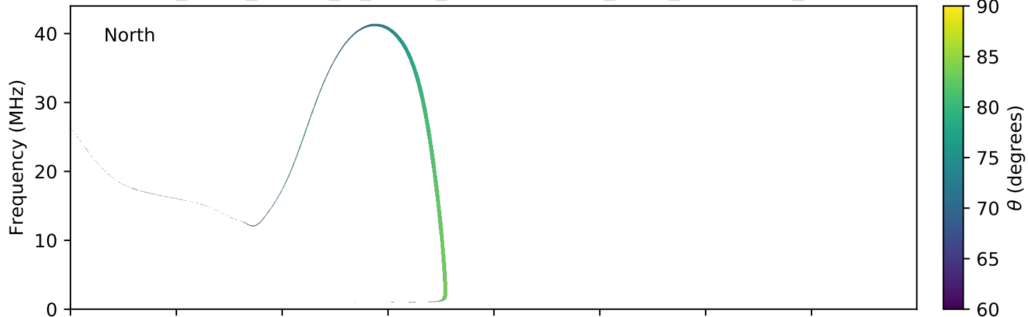
expres_earth_jupiter_io_jrm09_lossc-wid1deg_3kev_20120206_v01.cdf
