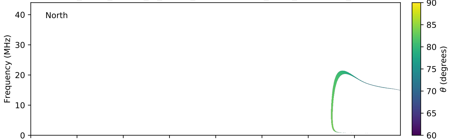
expres_earth_jupiter_io_jrm09_lossc-wid1deg_3kev_20120203_v01.cdf
