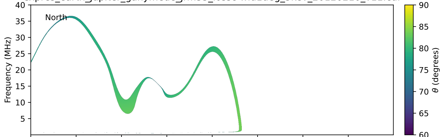
expres_earth_jupiter_ganymede_jrm33_lossc-wid1deg_3kev_20120210_v11.cdf
