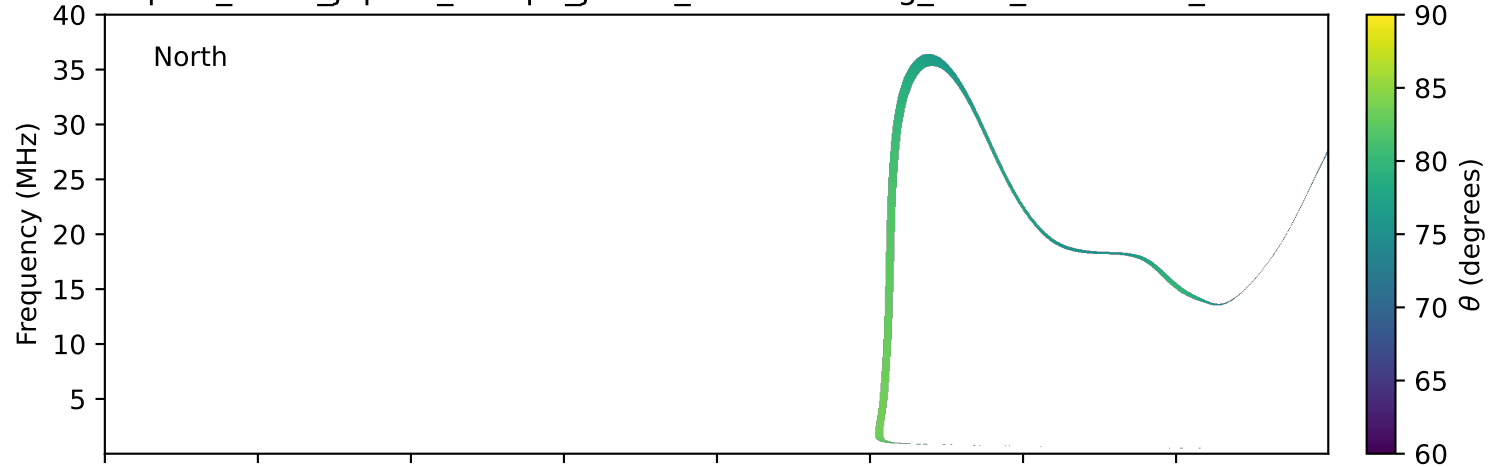
expres_earth_jupiter_europa_jrm33_lossc-wid1deg_3kev_20120218_v11.cdf
