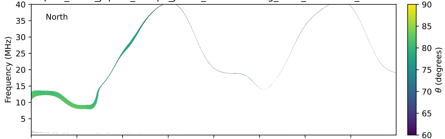
expres_earth_jupiter_europa_jrm33_lossc-wid1deg_3kev_20120215_v11.cdf
