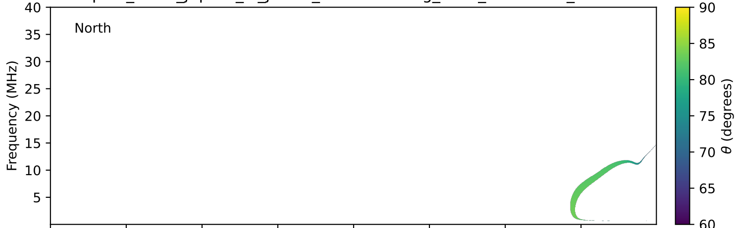
expres_earth_jupiter_io_jrm33_lossc-wid1deg_3kev_20111203_v11.cdf
