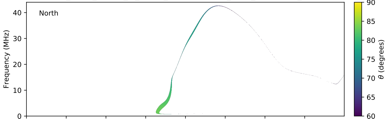
expres_earth_jupiter_io_jrm09_lossc-wid1deg_3kev_20111230_v01.cdf
