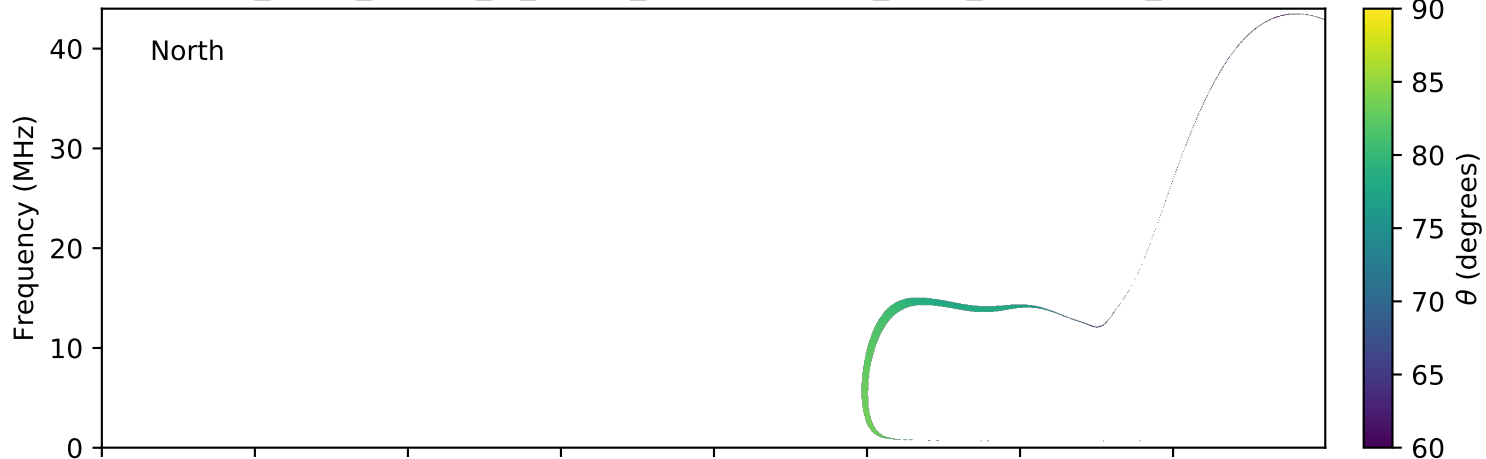
expres_earth_jupiter_io_jrm09_lossc-wid1deg_3kev_20111228_v01.cdf
