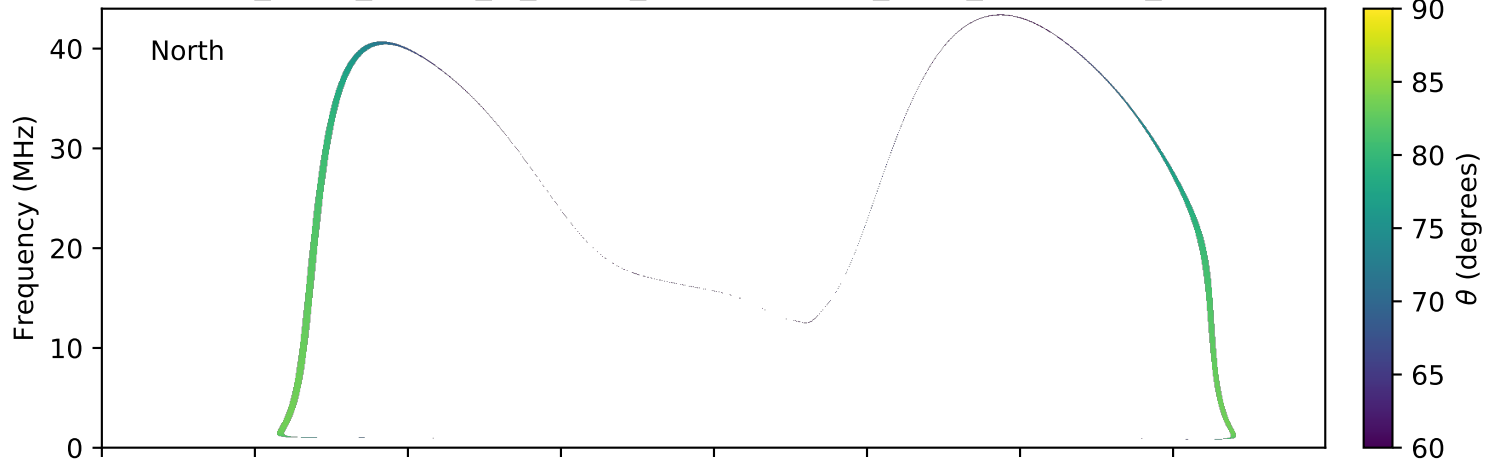
expres_earth_jupiter_io_jrm09_lossc-wid1deg_3kev_20111225_v01.cdf
