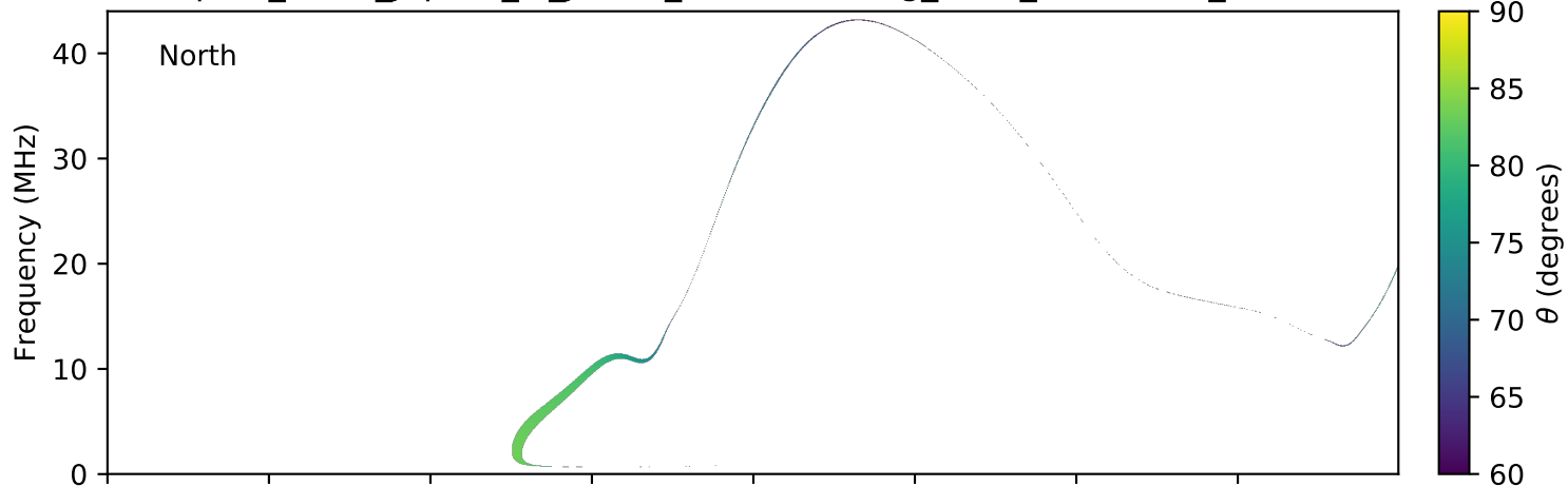
expres_earth_jupiter_io_jrm09_lossc-wid1deg_3kev_20111223_v01.cdf
