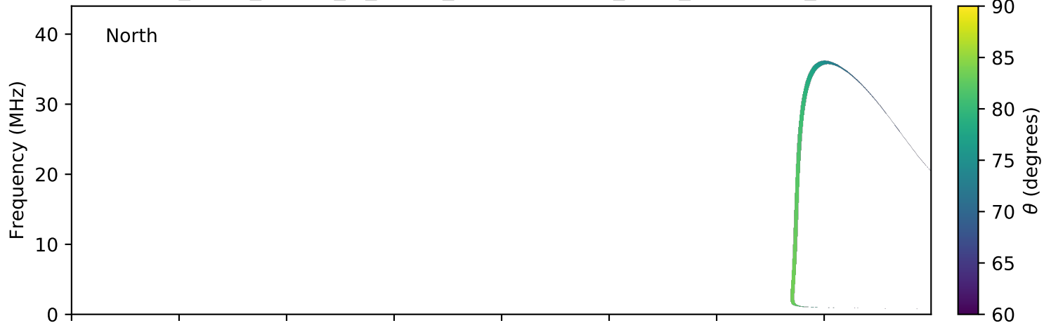
expres_earth_jupiter_io_jrm09_lossc-wid1deg_3kev_20111219_v01.cdf
