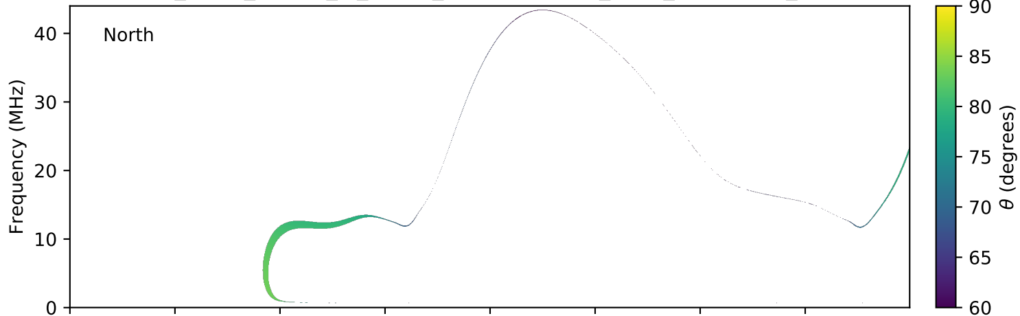
expres_earth_jupiter_io_jrm09_lossc-wid1deg_3kev_20111216_v01.cdf
