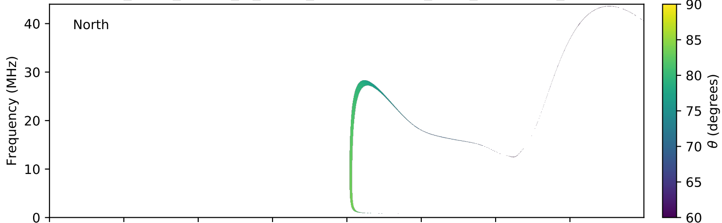
expres_earth_jupiter_io_jrm09_lossc-wid1deg_3kev_20111214_v01.cdf
