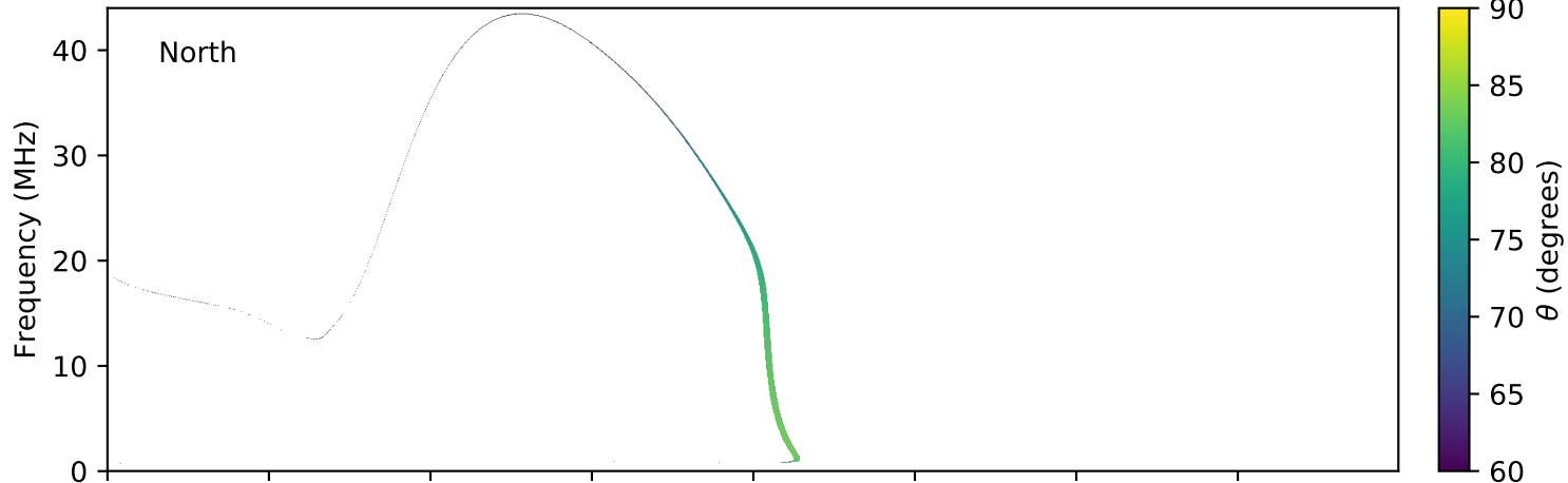
expres_earth_jupiter_io_jrm09_lossc-wid1deg_3kev_20111213_v01.cdf
