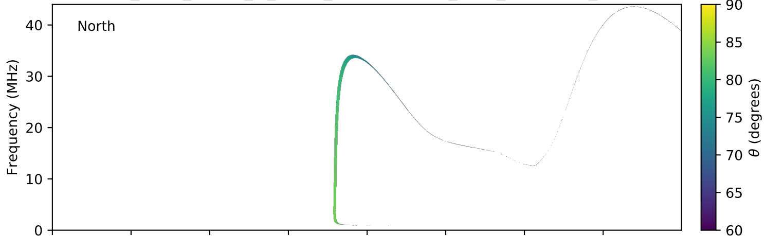
expres_earth_jupiter_io_jrm09_lossc-wid1deg_3kev_20111207_v01.cdf
