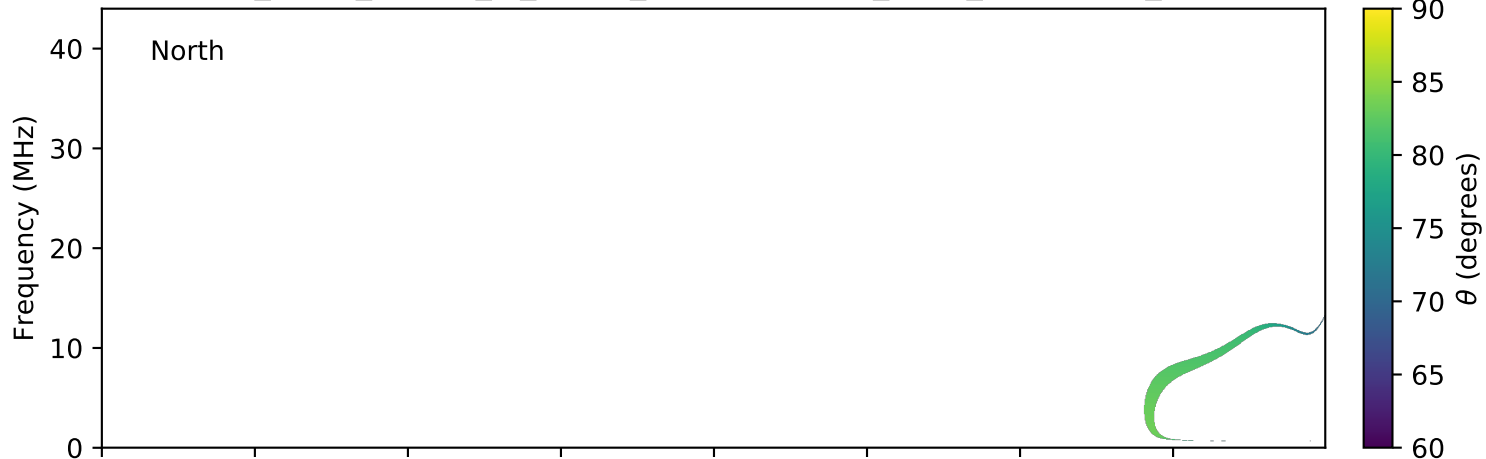
expres_earth_jupiter_io_jrm09_lossc-wid1deg_3kev_20111203_v01.cdf
