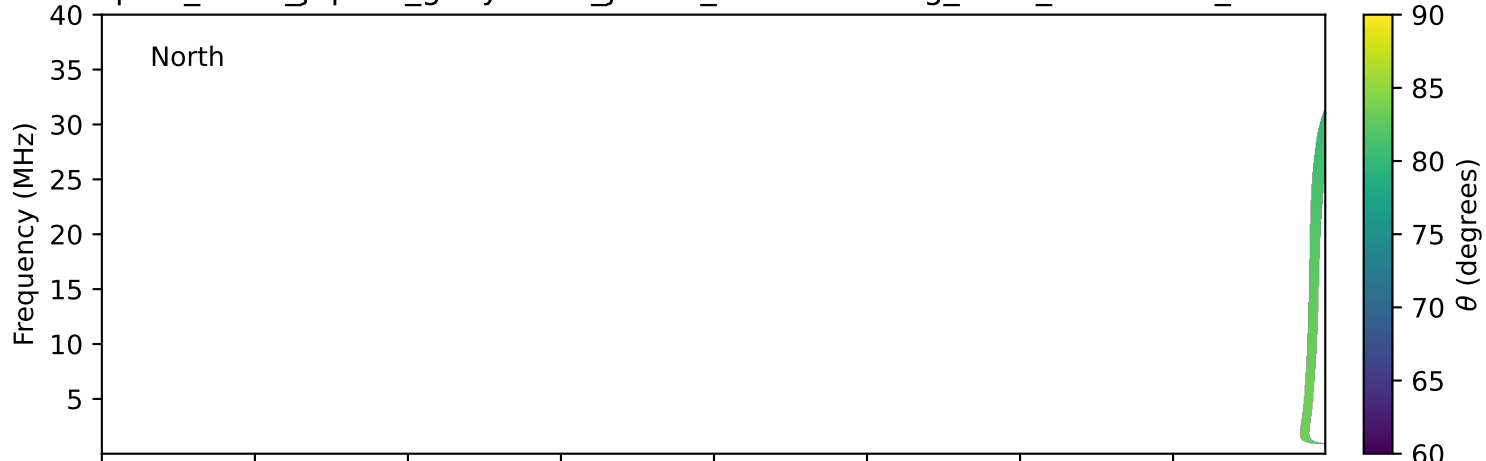
expres_earth_jupiter_ganymede_jrm33_lossc-wid1deg_3kev_20111211_v11.cdf
