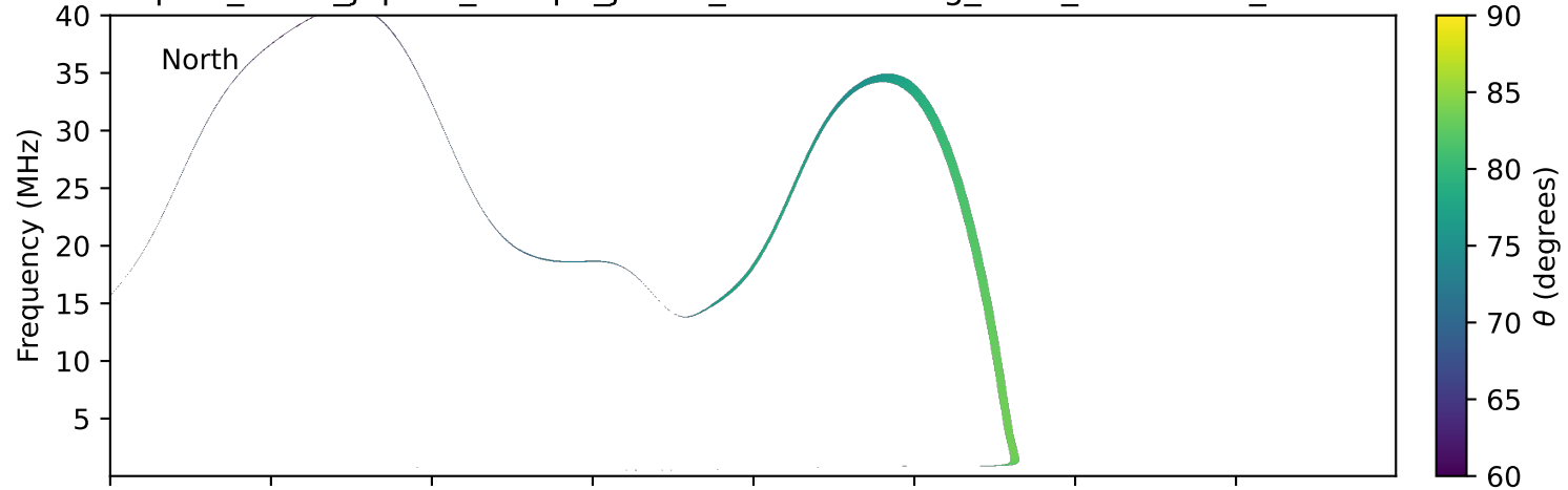
expres_earth_jupiter_europa_jrm33_lossc-wid1deg_3kev_20111214_v11.cdf
