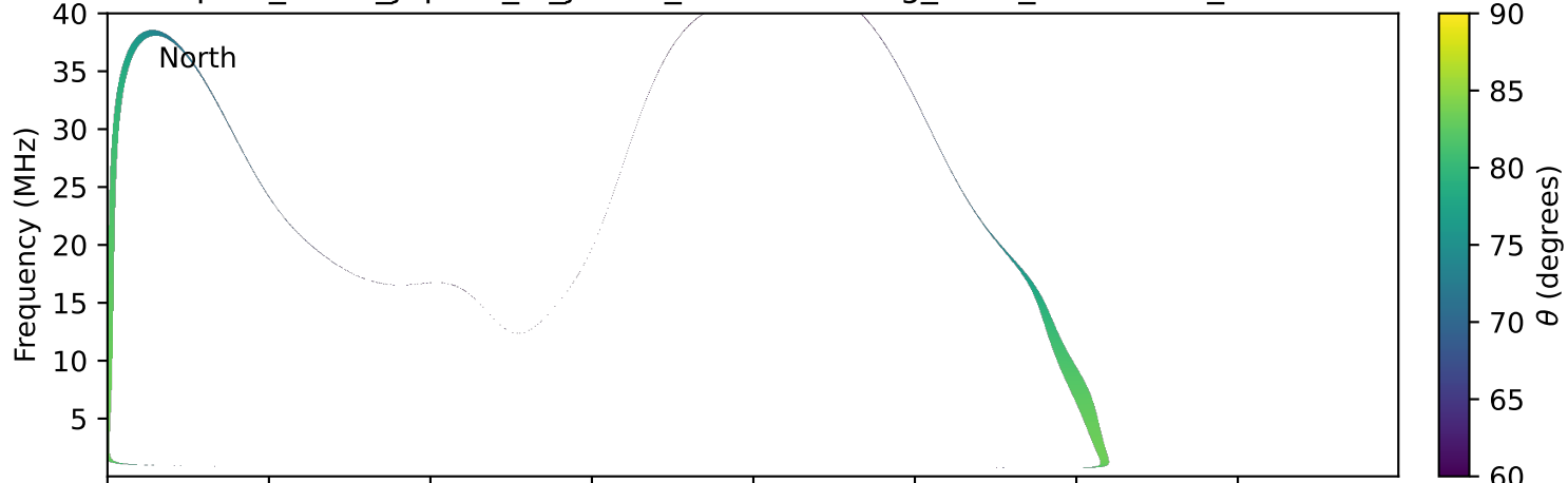
expres_earth_jupiter_io_jrm33_lossc-wid1deg_3kev_20111118_v11.cdf
