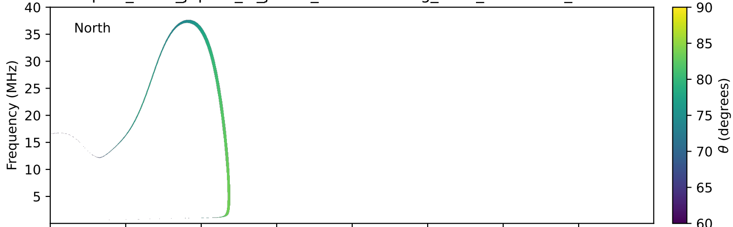
expres_earth_jupiter_io_jrm33_lossc-wid1deg_3kev_20111115_v11.cdf
