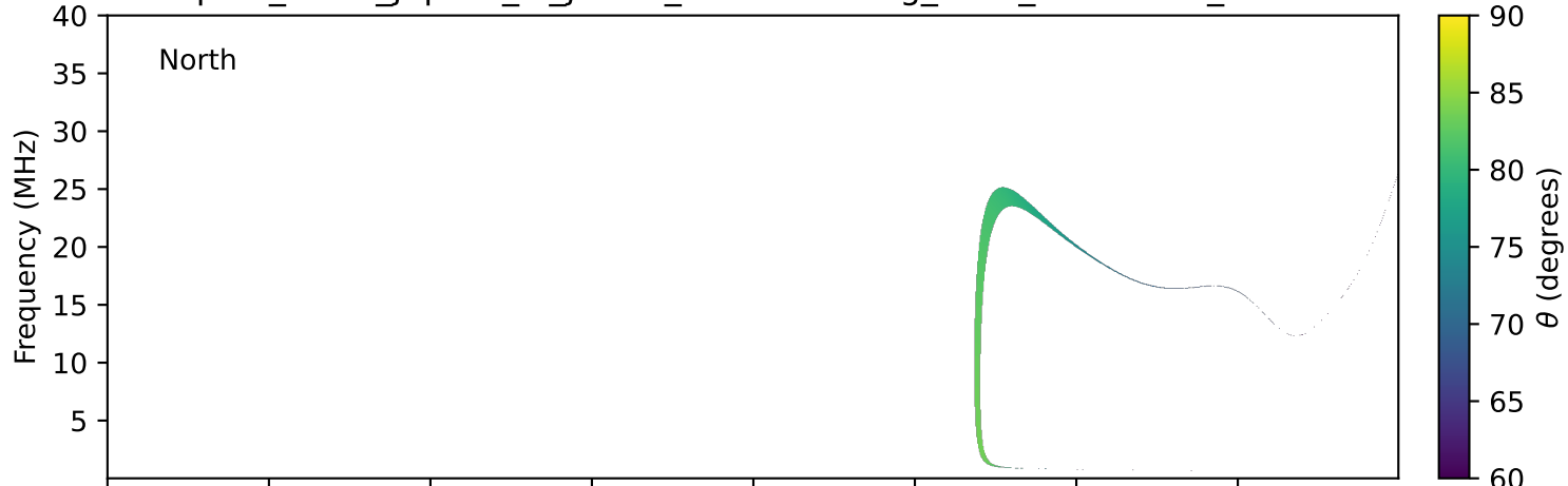
expres_earth_jupiter_io_jrm33_lossc-wid1deg_3kev_20111112_v11.cdf
