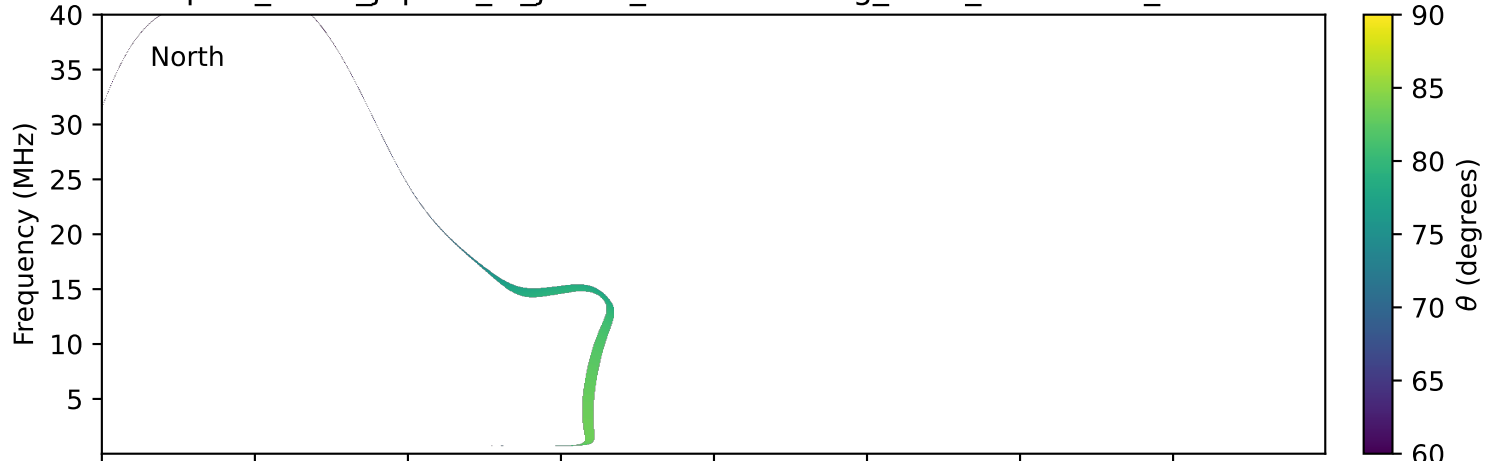
expres_earth_jupiter_io_jrm33_lossc-wid1deg_3kev_20111106_v11.cdf
